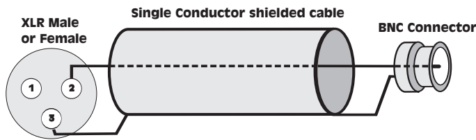
Figure 3-18. Unbalanced connections using single-conductor cable
