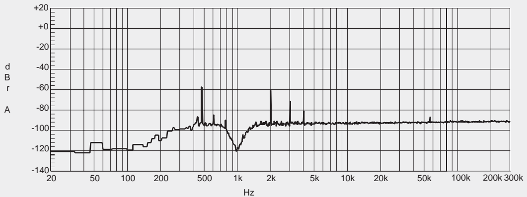
Figure 4-12. Spectrum with 400 Hz bandpass filter applied
